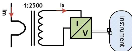
Figure 3: A 1398 PQA Iron Current Clamp - block diagram
