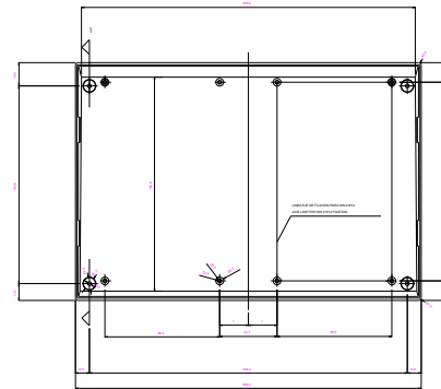
BASE: PLANTA INTERIOR BOTTOM: INSIDE VIEW
