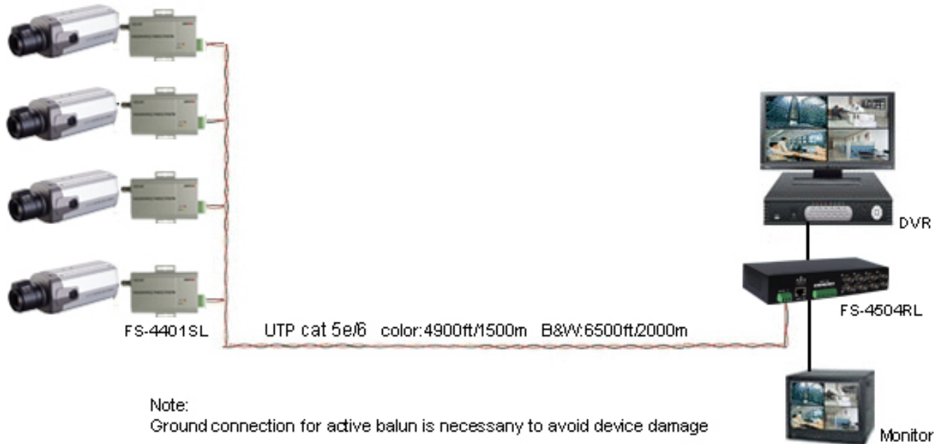
Diagram 3 FS-4401SL + FS-4504RL
