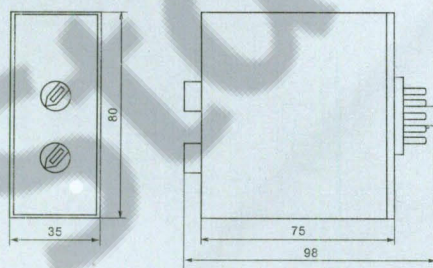
AS-CP1 Outline dimension
