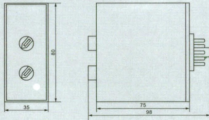
AS-PT1 Outline dimension
