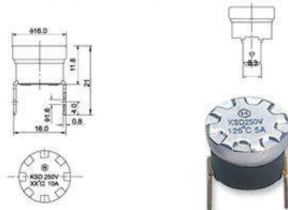
(W/O BVL) Without Bracket Vertical Lead
