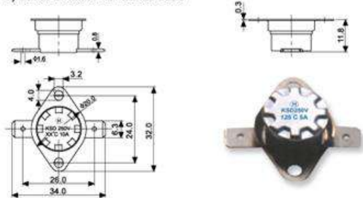
(LBHL) Loose Bracket Horizontal Lead
