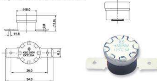
(W/O BHL) Without Bracket Horizontal Lead
