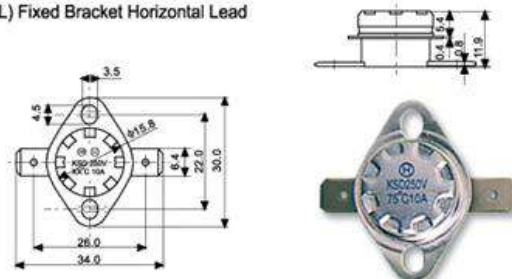
(FBHL) Fixed Bracket Horizontal Lead
