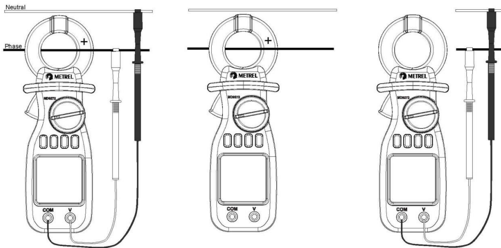
Measurement of power Measurement of current Measurement of voltage
