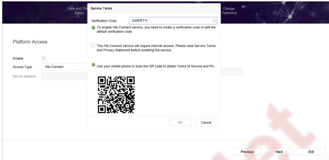
Figure 2-11 Hik-Connect Access
