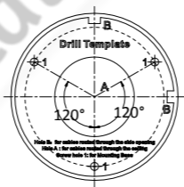
Figure 2-1 Drill Template
