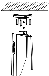
Figure 2-2 Install the Camera to the Ceiling
