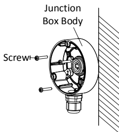
Figure 2-6 Secure the Box's Body to the Ceiling
