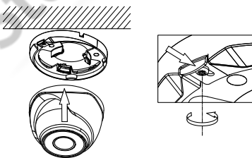
Figure 2-11 Install the Turret Camera
