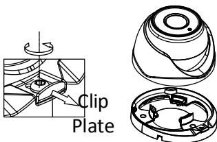
Figure 2-9 Remove the Clip Plate
