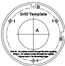
Figure 2-4 Drill Template
