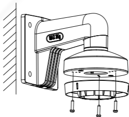
Figure 2-14 Install the Mounting Base to the Bracket
