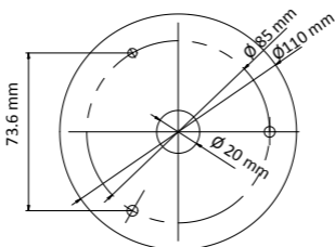
Figure 2-1 Drill Template
