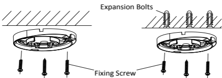
Figure 2-2 Attach the Mounting Base to the Ceiling
