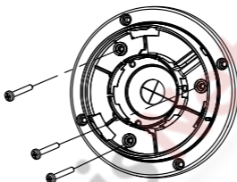
Figure 2-10 Install Turret Camera's Mounting Base
