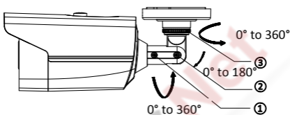
Figure 2-10 3-Axis Adjustment
