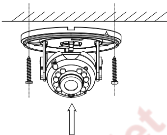
Figure 2.11 Attach the Mounting Base to the Ceiling
