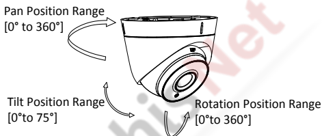
Figure 2. 8 3-axis Adjustment
