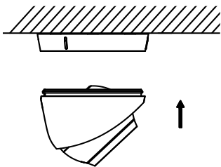
Figure 2. 7 Secure the Camera with Mounting Base
