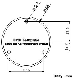
Figure 2. 1 Drill Template
