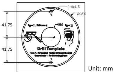
Figure 2.10 Drill Template
