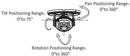
Figure 2.12 3-axis Adjustment
