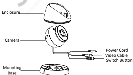
Figure 1. 2 Type II Camera Overview
