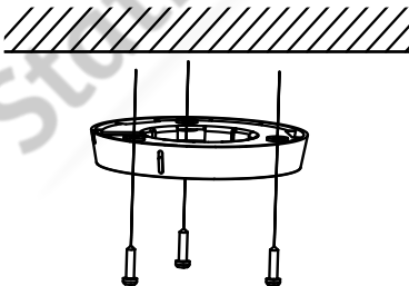
Figure 2. 6 Attach the Mounting Base to the Ceiling
