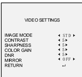
Figure 3. 6 VIDEO SETTINGS
