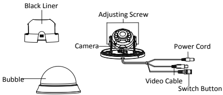
Figure 1. 3 Type III Camera Overview
